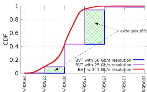
Fig. 4. Cumulative percentage of channels that can be upgraded to faster modulations using 50, 25, and 1 Gb/s resolution.
