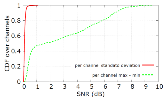
Fig. 8. CDF of SNR variation over time for each channel.
